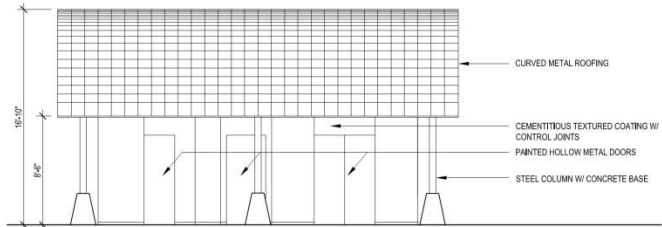
ELEVATION WEST
