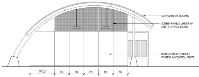
ELEVATION SOUTH
