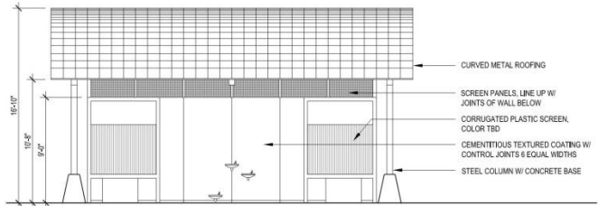
ELEVATION EAST
