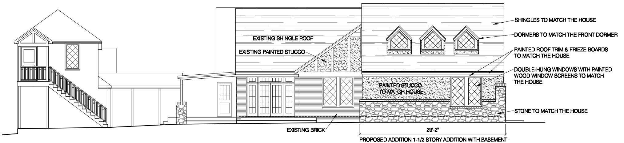
AFTER - Side (South) Elevation 1/8" = 1'-0"
