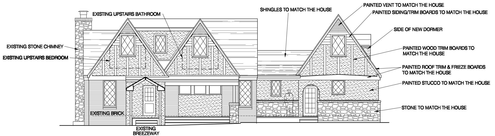
AFTER - Back (West) Elevation 1/8" = 1'-0"
