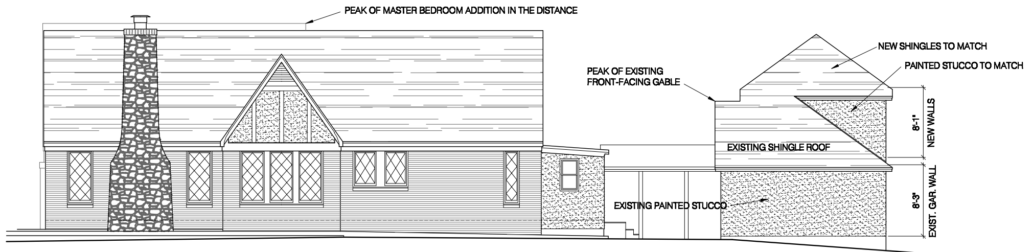
AFTER - Side (North) Elevation 1/8" = 1'-0"
