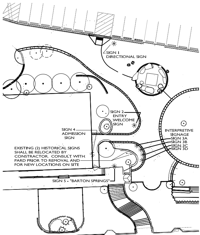
NORTH POOL ENTRANCE - SIGN LOCATION PLAN SCALE 1"=20'-0"
