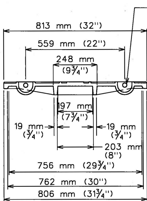
LID SECTION VIEW
