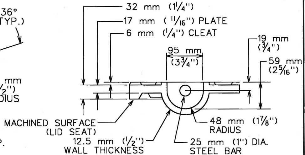
PICK BAR DETAIL
