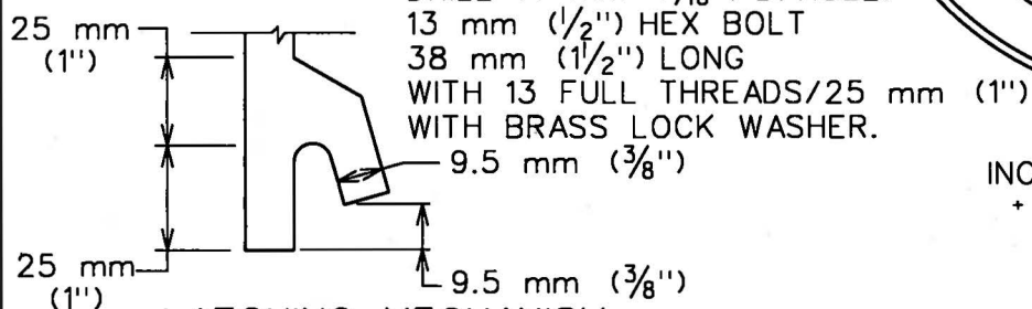
LATCHING MECHANISM
