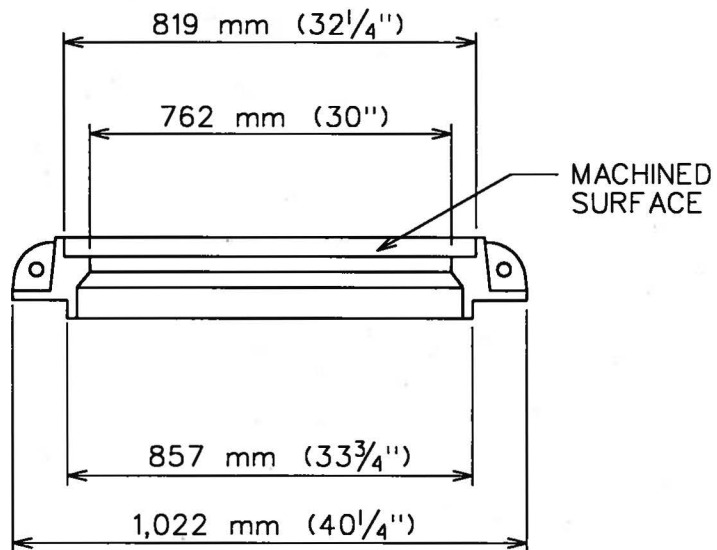
RING SECTION
