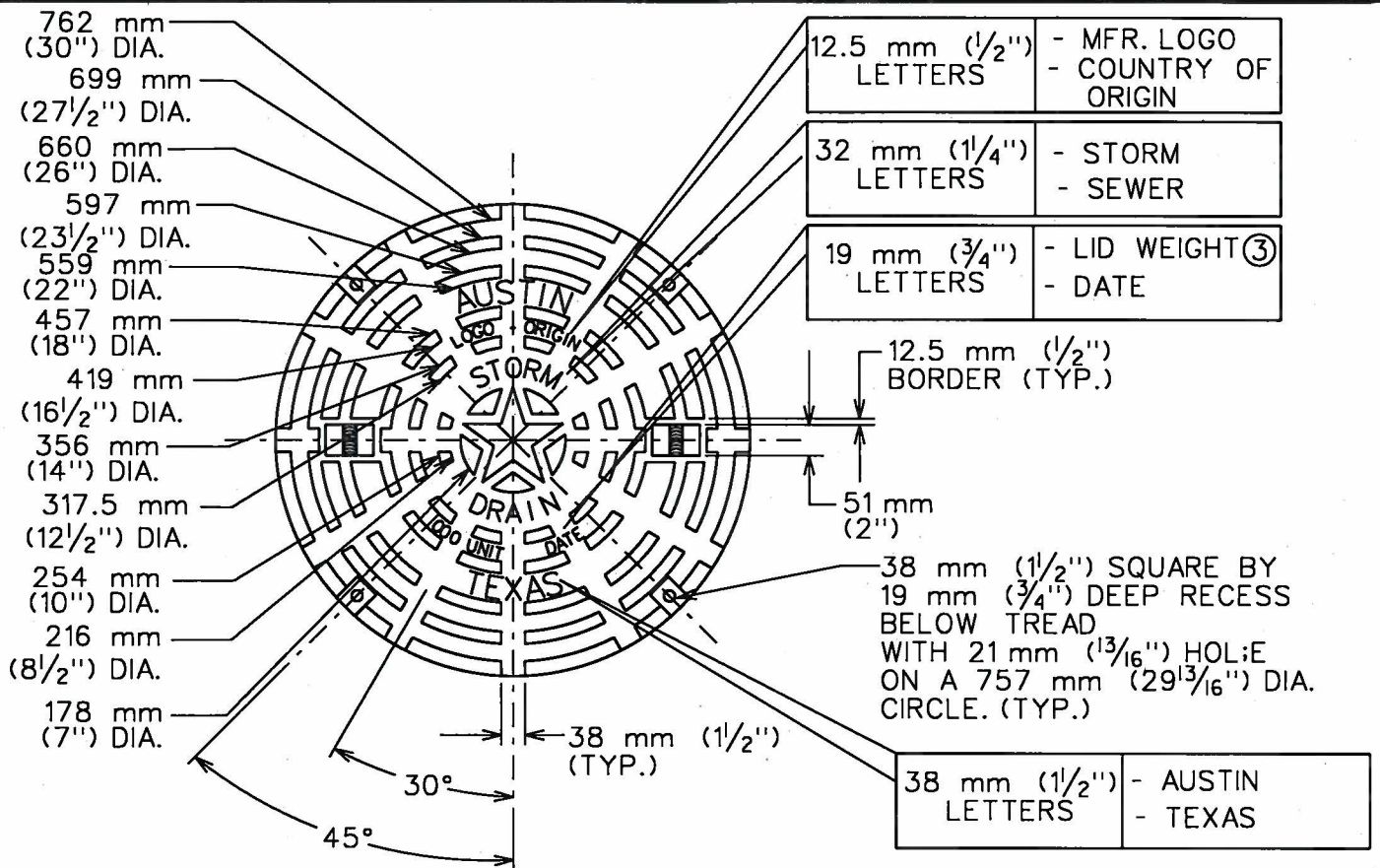
LID PLAN VIEW
