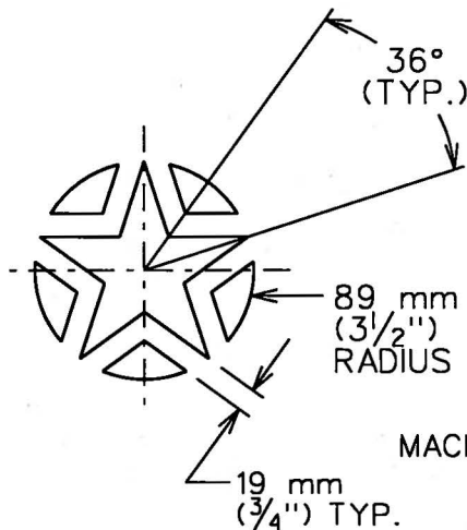
STAR LAYOUT
