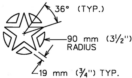
STAR LAYOUT
