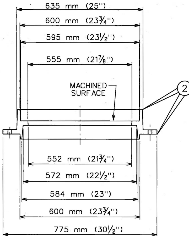
RING SECTION
