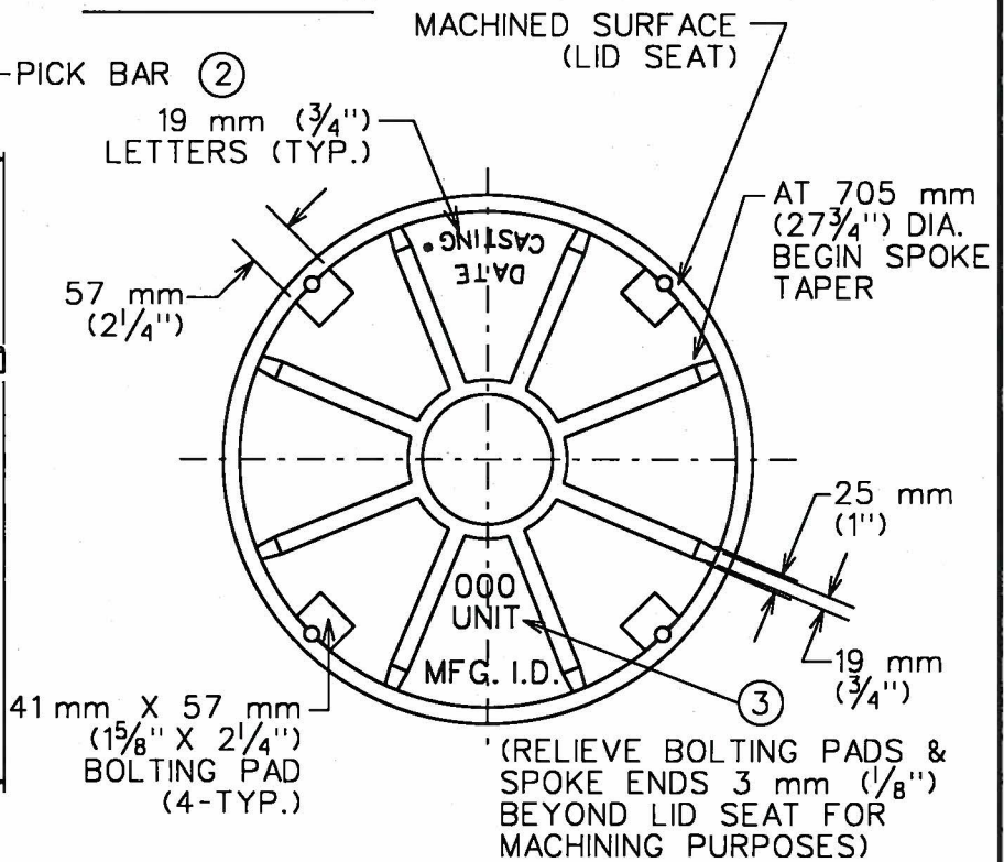
LID SECTION VIEW
