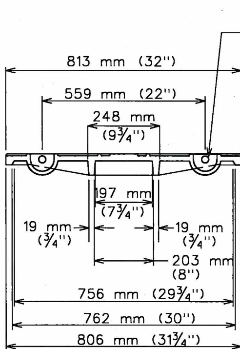
LID SECTION VIEW
