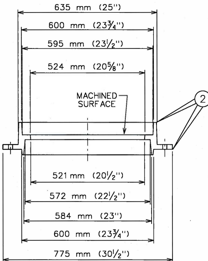
RING SECTION
