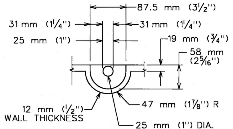
PICK BAR DETAIL
