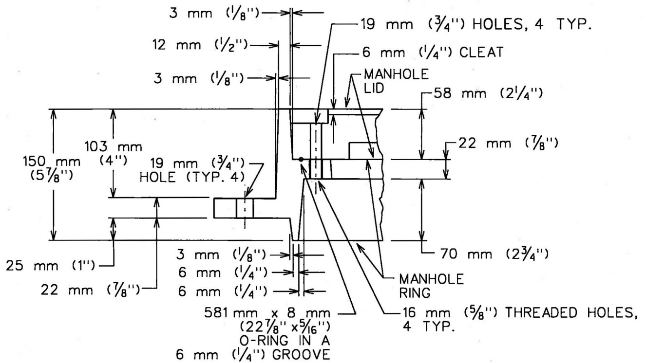
BOLT HOLE AND WATER-TIGHT DETAIL
