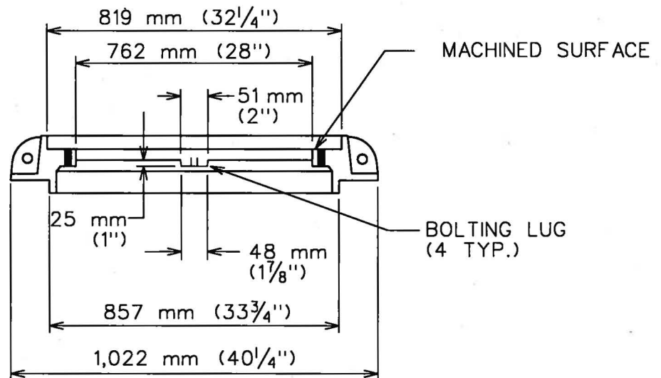
RING SECTION
