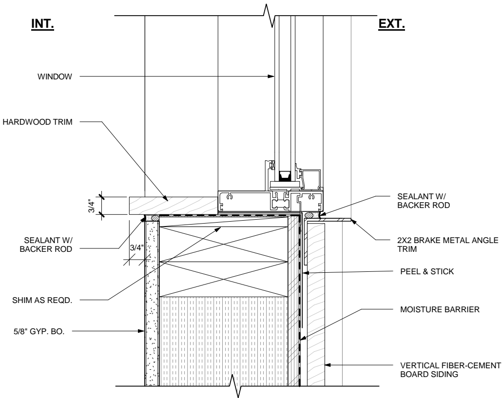
WINDOW TYP. SILL
