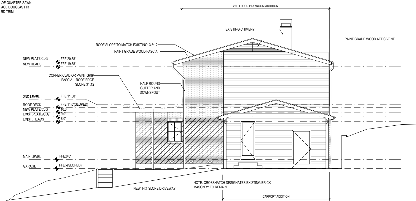
2 NEW NORTH SIDE ELEVATION SCALE: 3/16" = 1'-0"
