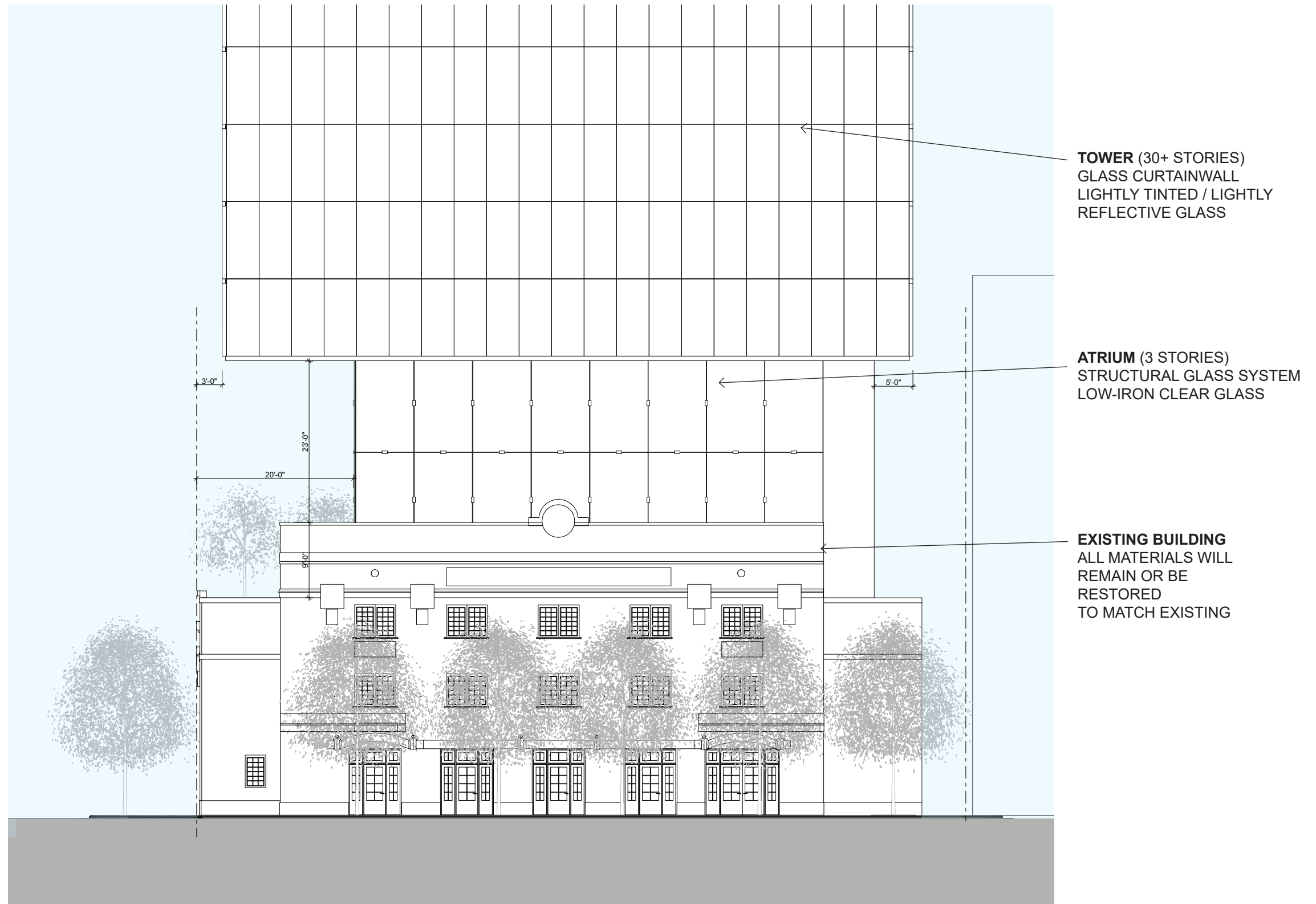
NORTH ELEVATION
