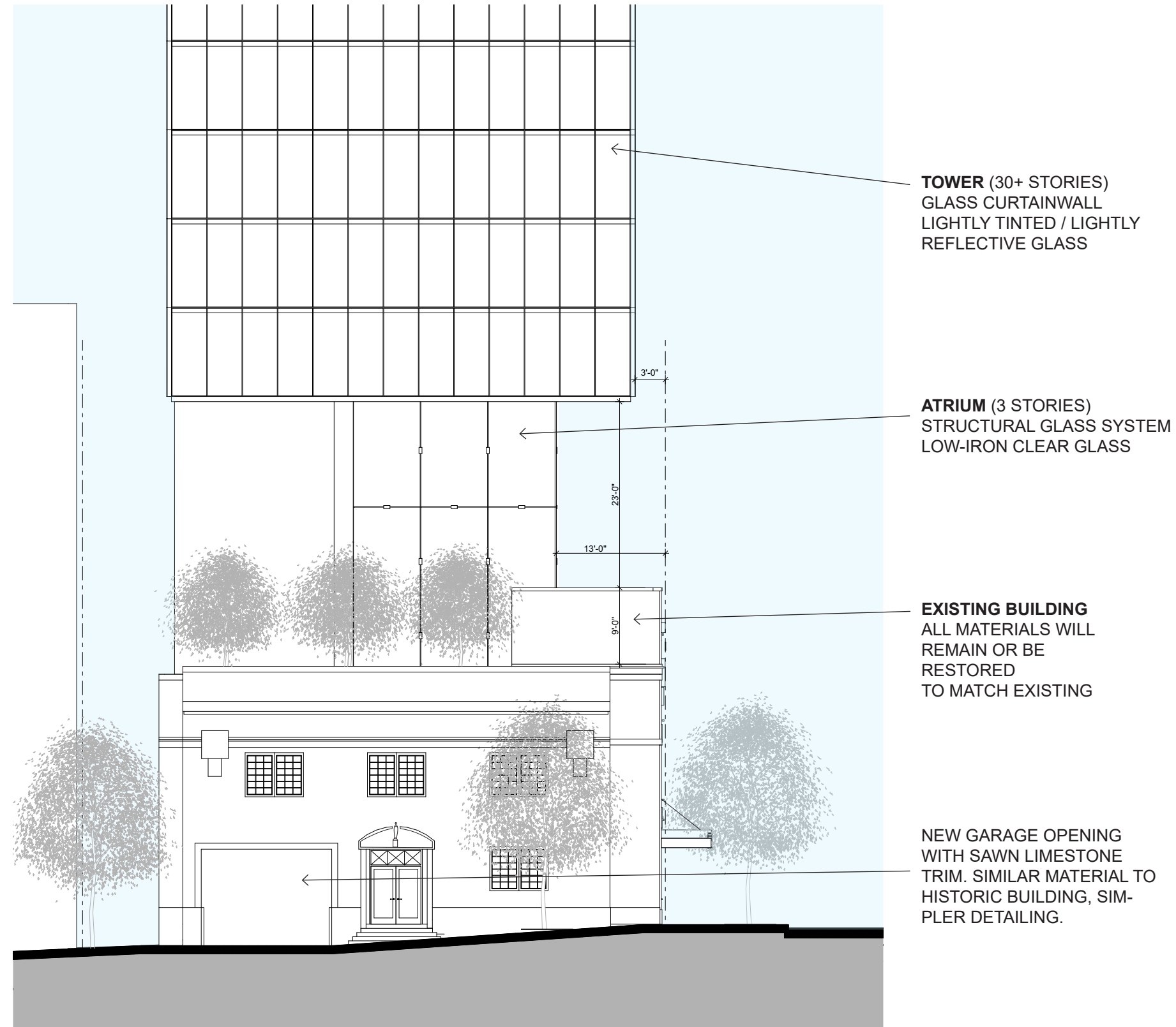
EAST ELEVATION
