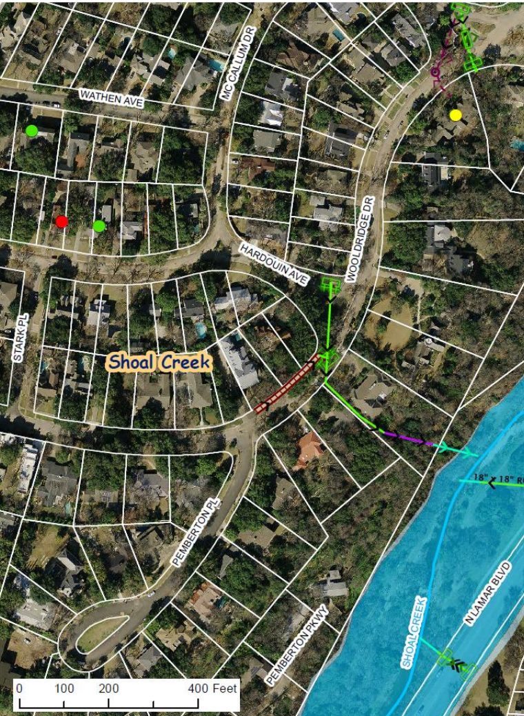
Existing Storm Drain System
