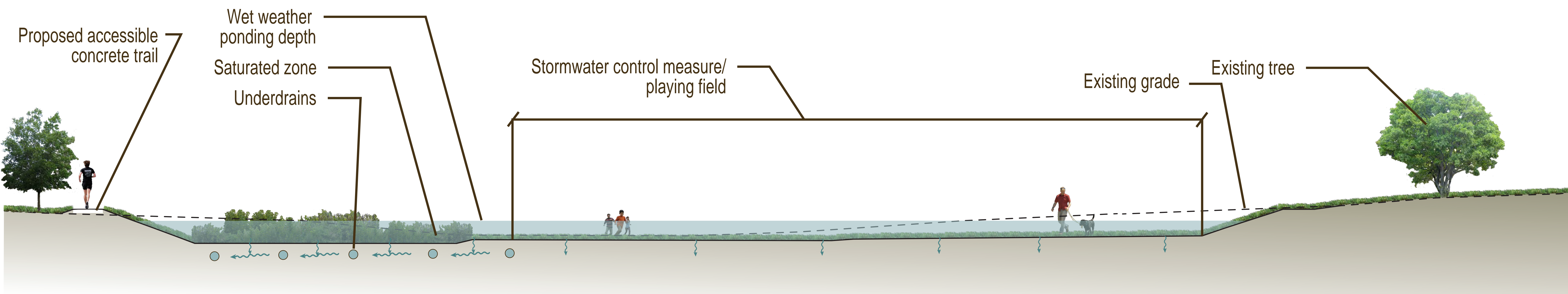
Section Through Stormwater Control Measure Looking West
