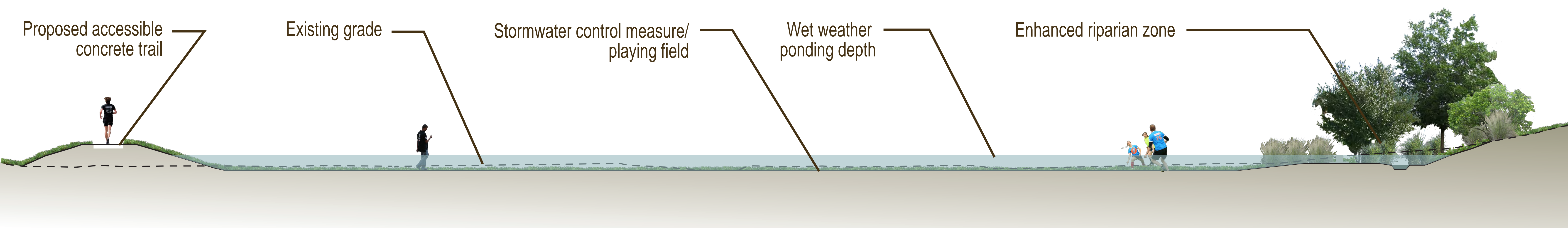
Section Through Stormwater Control Measure and Riparian Zone Looking South
