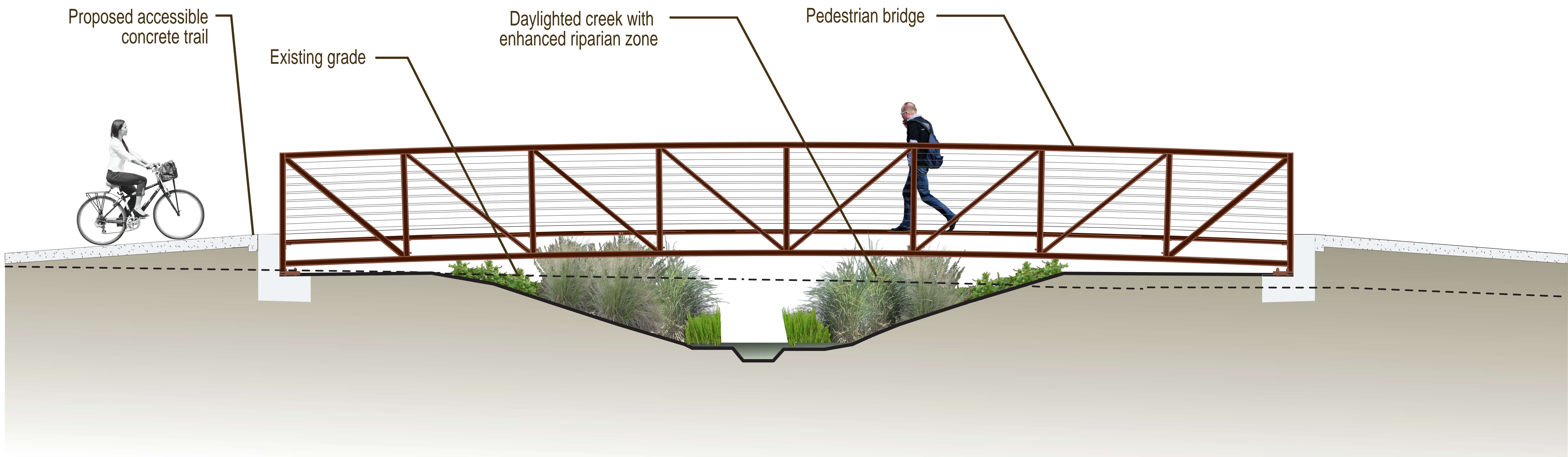
Section Through Daylighted Creek
