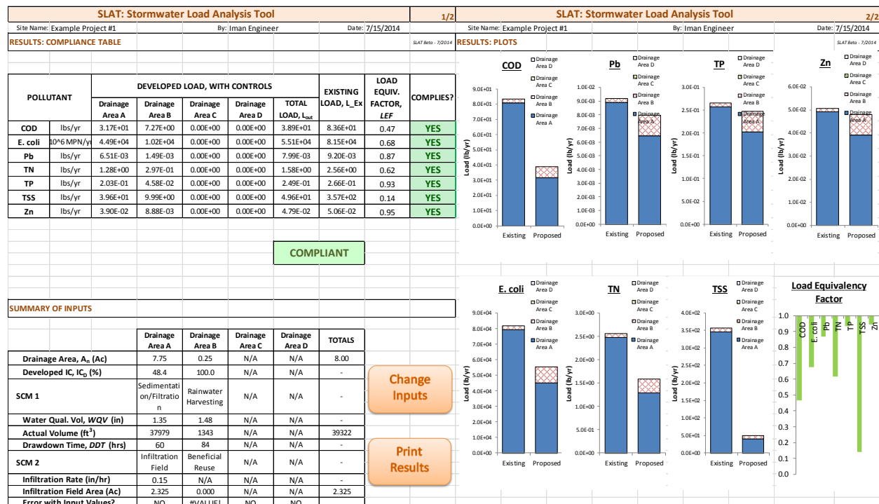
Figure 7: Screenshot of worksheet “2. RESULTS” showing that updated proposed design, with modified drawdown time and water quality volume for Drainage Area 1, complies with SOS load requirements.
