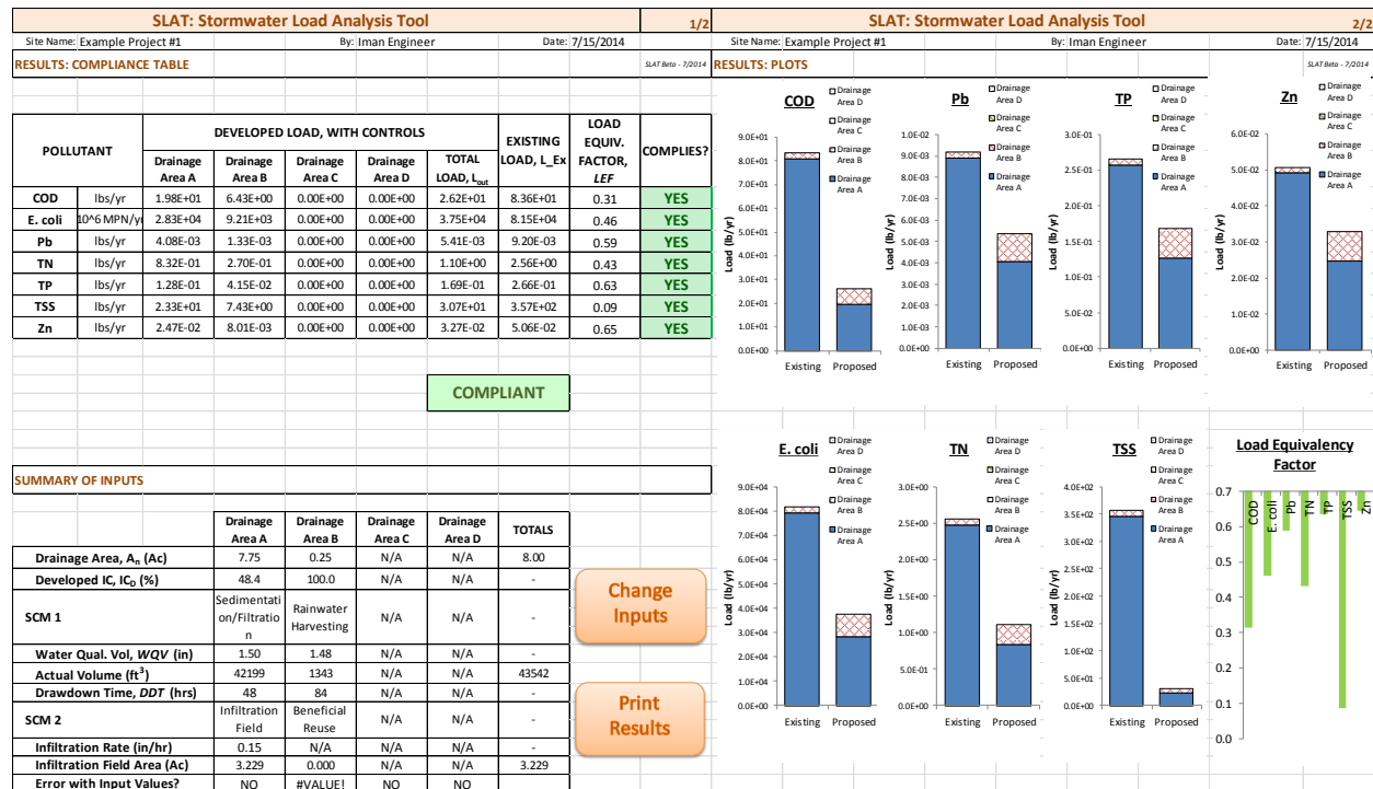
Figure 6: Screenshot of worksheet “2. RESULTS” showing that proposed design complies with SOS requirements.
