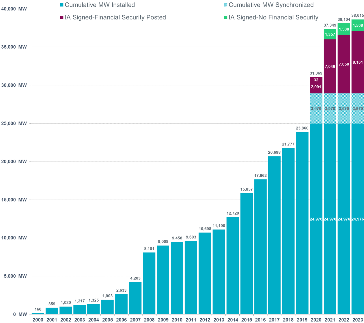
ERCOT Wind Additions by Year (as of Aug 31, 2020)
