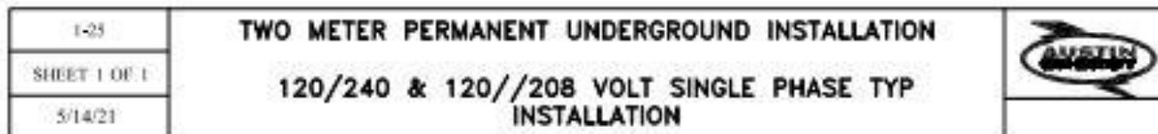
Figure 1-25. Two-Meter Permanent Underground Installation (Typical Installation)
