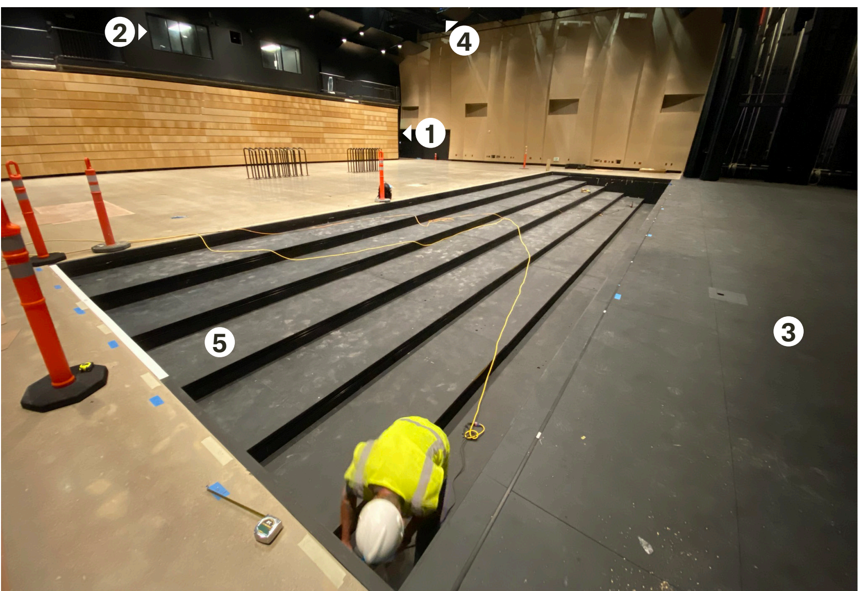
Adjustable Floor
