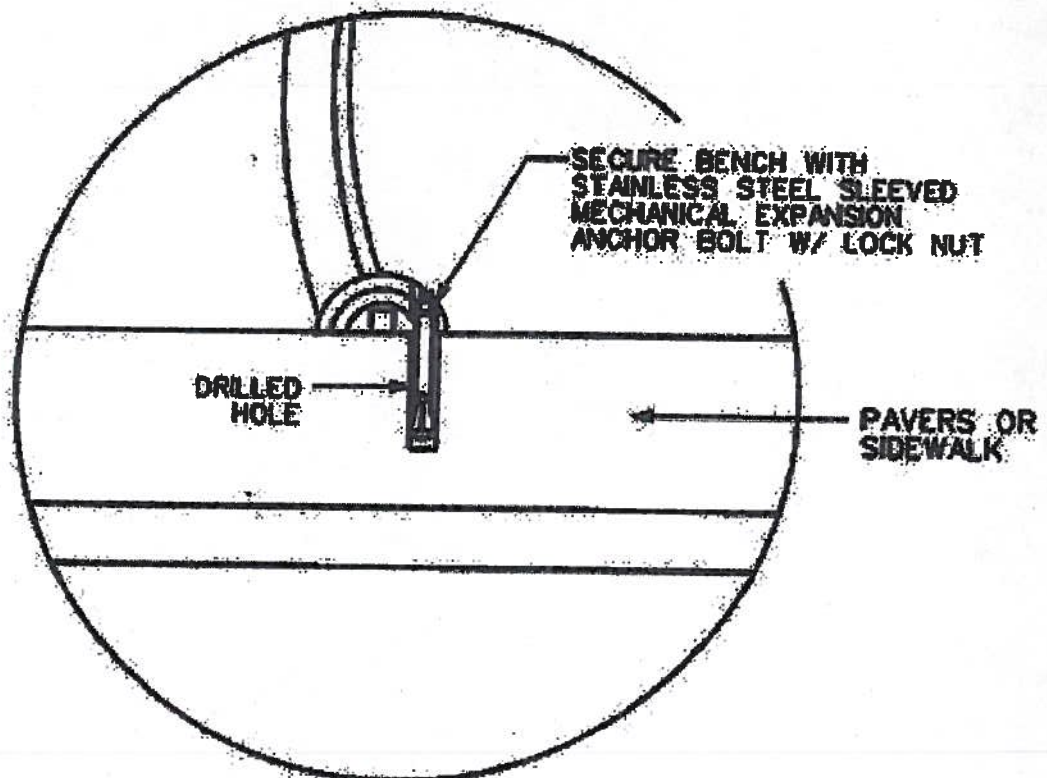
INSTALLATION DETAIL
