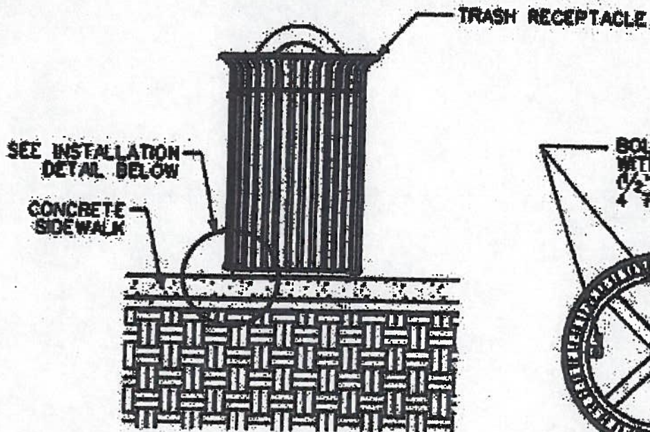
BASIC INSTALLATION
