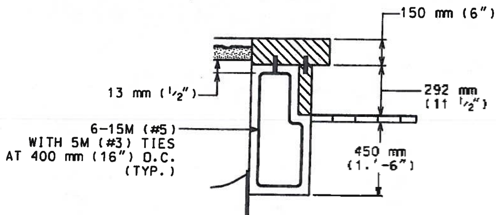
SECTION B
