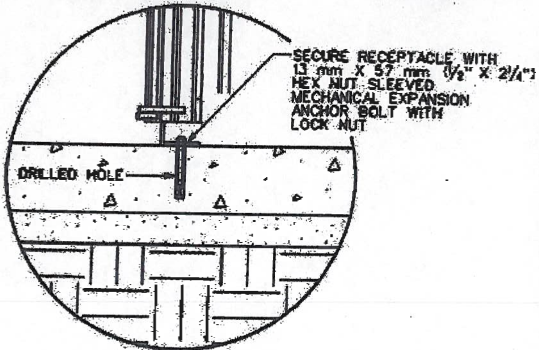
INSTALLATION DETAIL
