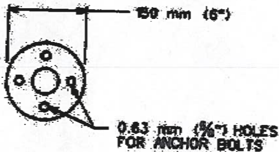
ANCHOR DETAIL
