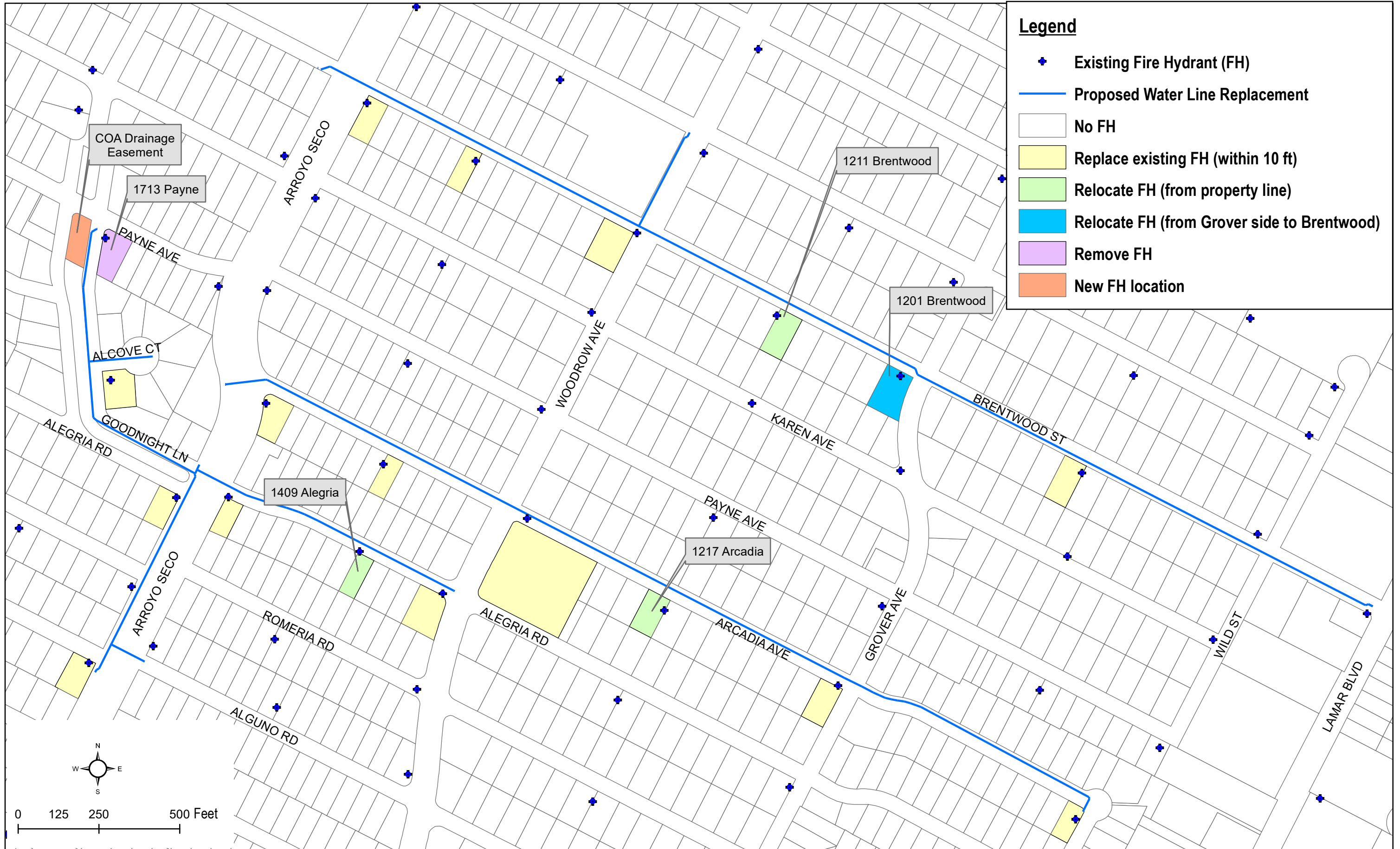
2231.233 - Brentwood Water & Wastewater Pipeline Renewal: Arcadia Ave. Area - Proposed Fire Hydrant Locations
