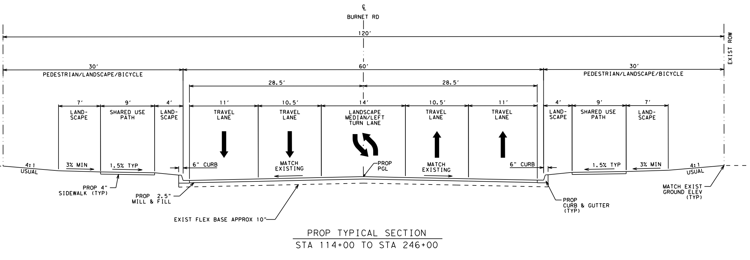
PROPOSED TYPICAL SECTION BURNET RD STA 114+00 TO STA 246+00
