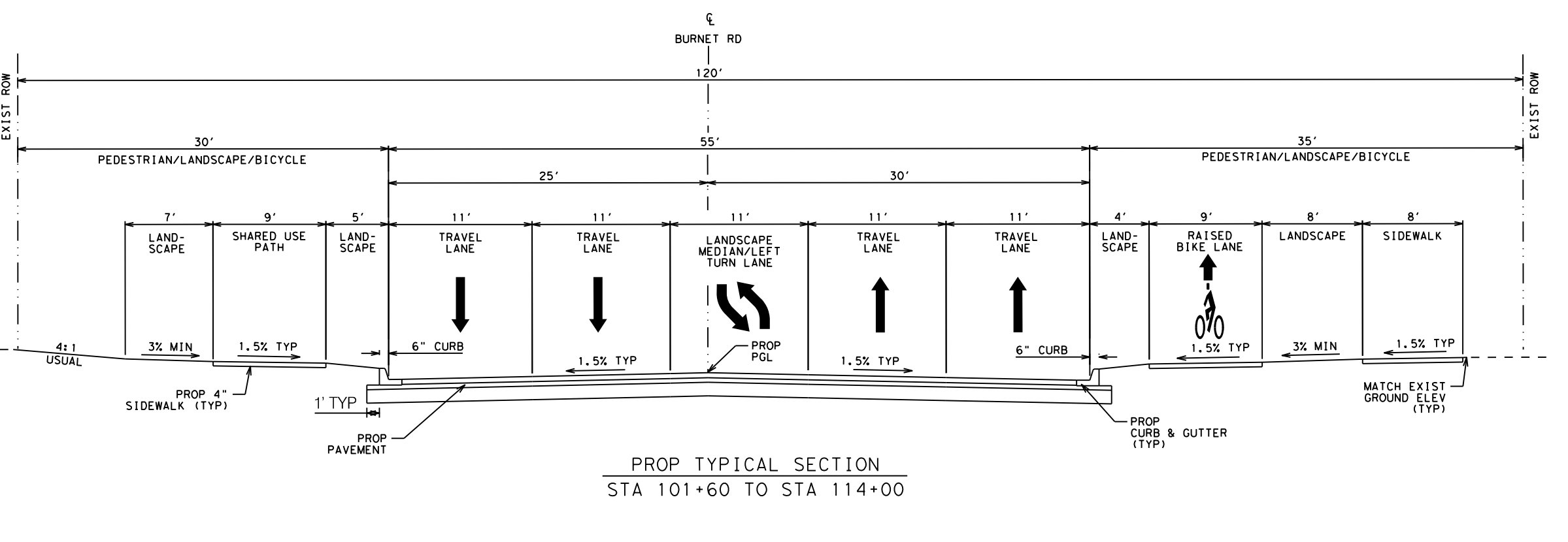
PROPOSED TYPICAL SECTION BURNET RD STA 101+60 TO STA 114+00
