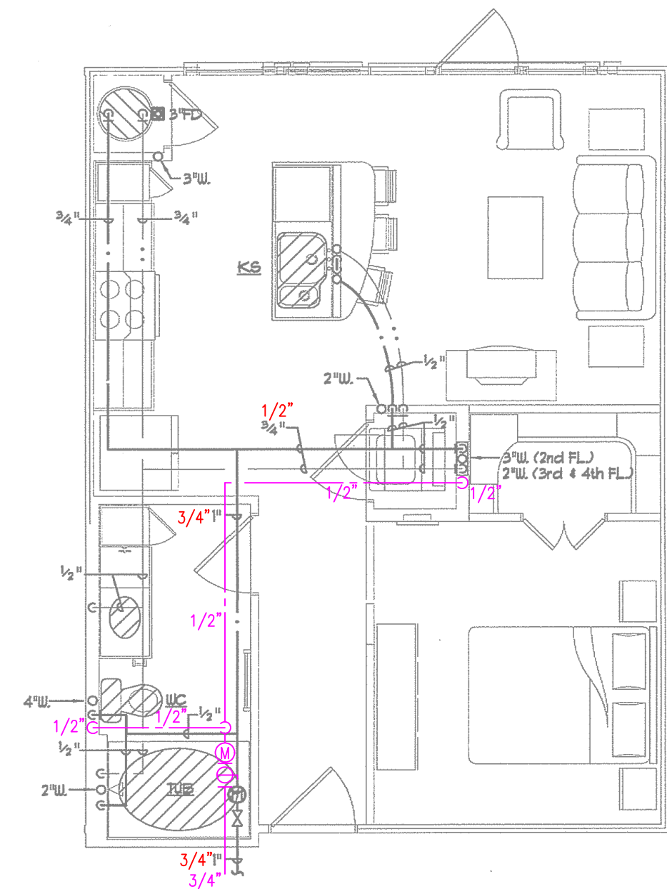
1 UNIT PLAN - S1A1 - PLUMBING SCALE: 1/4" = 1'-0"
