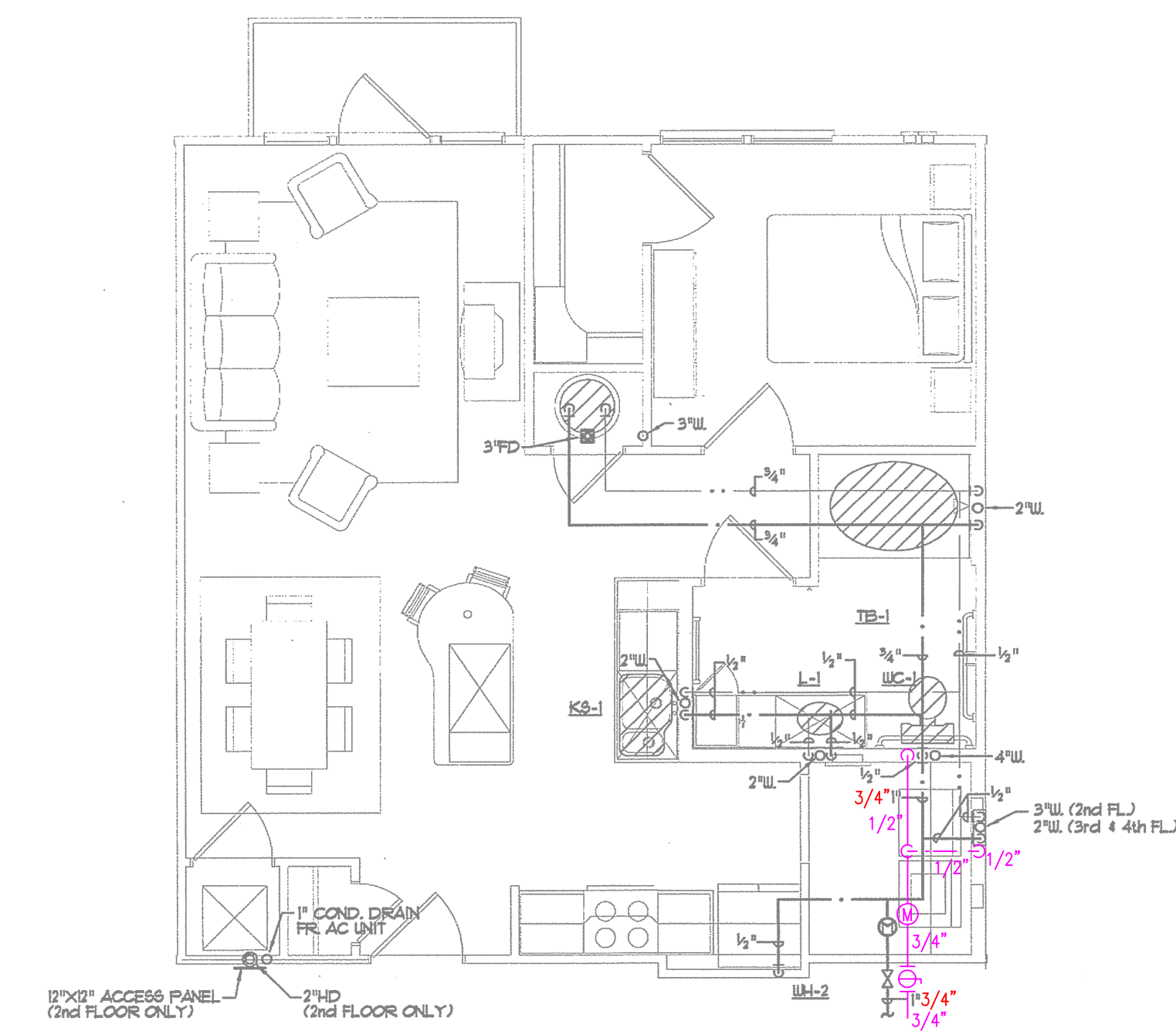
3 UNIT PLAN - A1BHC - PLUMBING SCALE: 1/4" = 1'-0"
