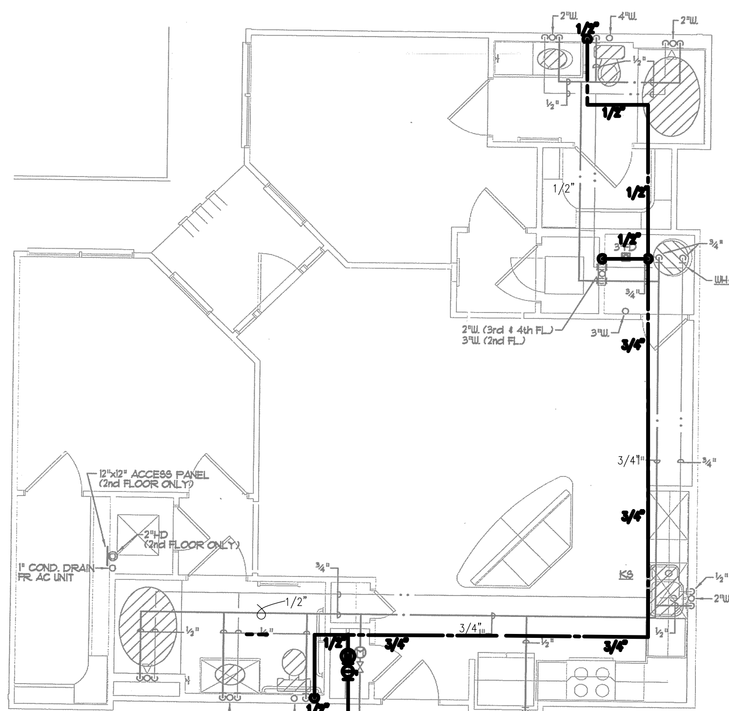
2 UNIT PLAN - B1A ANSI TYPE A - PLUMBING SCALE: 1/4" = 1'-0"
