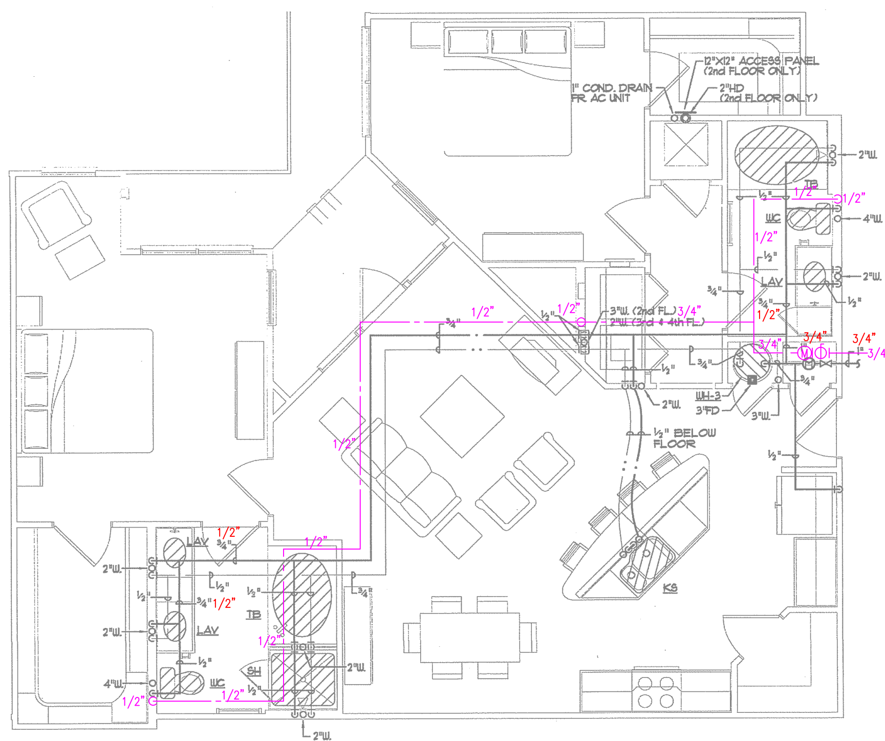
1 UNIT PLAN - B2H - PLUMBING SCALE: 1/4" = 1'-0"
