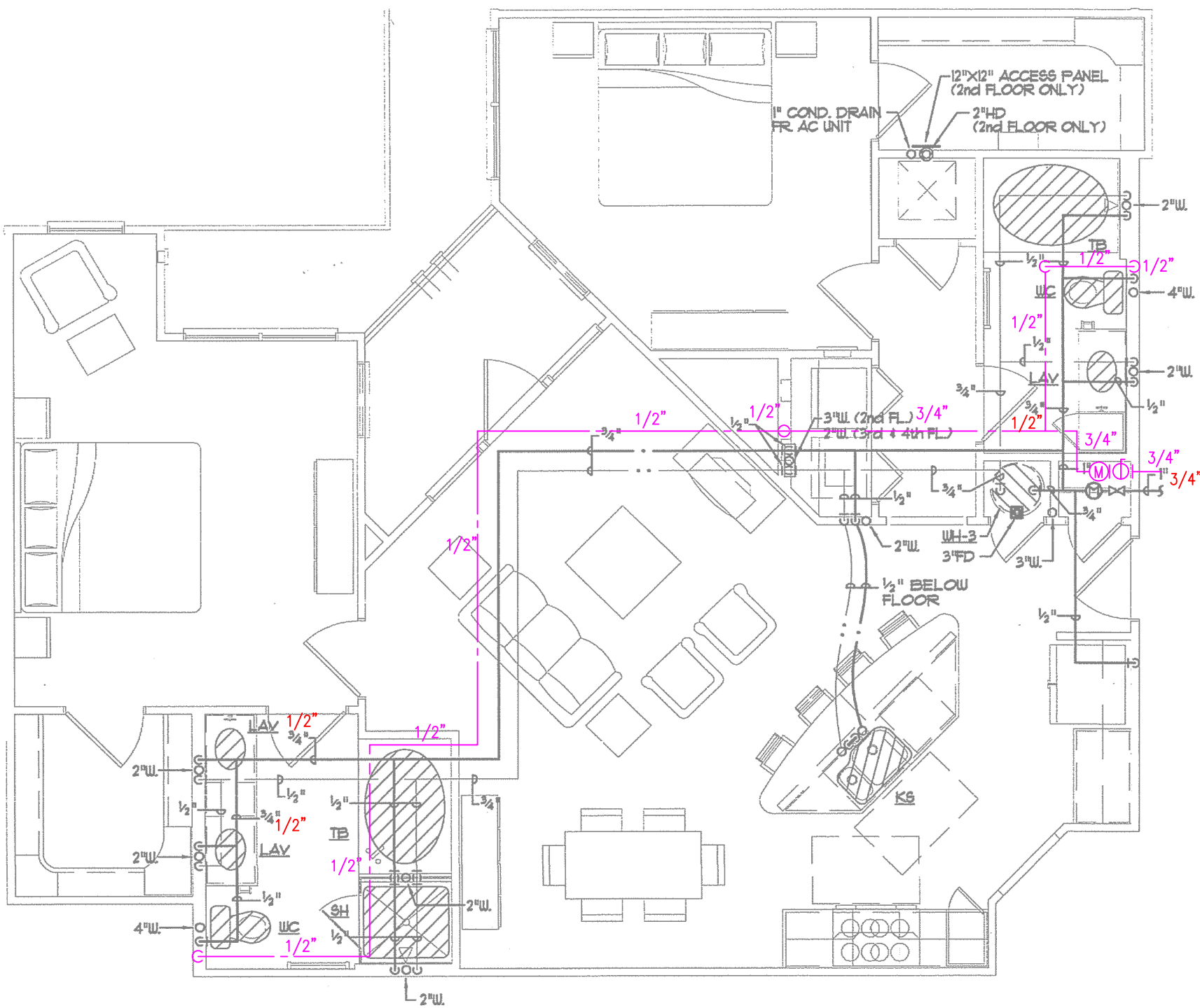
2 UNIT PLAN - B2B - PLUMBING SCALE: 1/4" = 1'-0"
