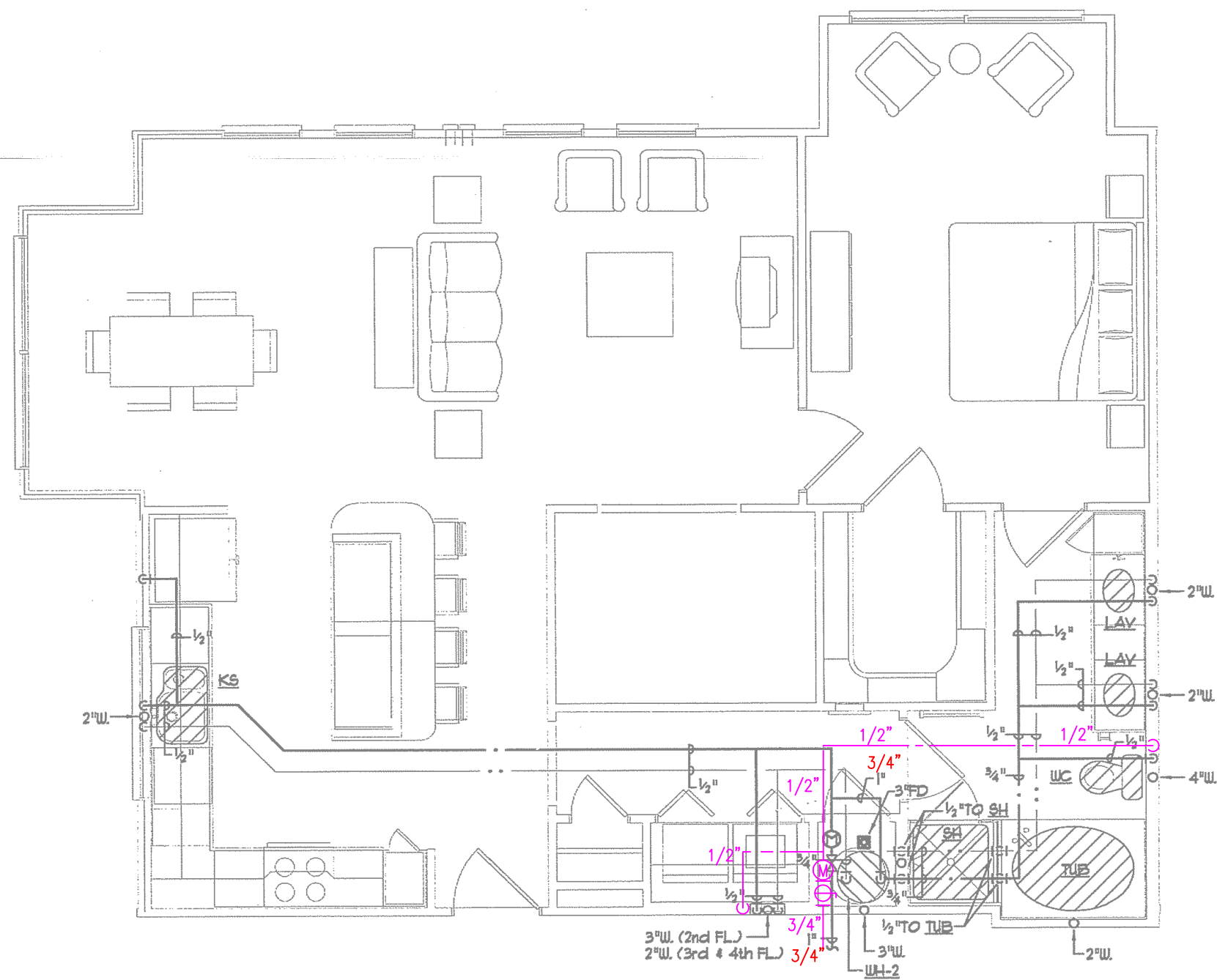
1 UNIT PLAN - A3D - PLUMBING SCALE: 1/4" = 1'-0"
