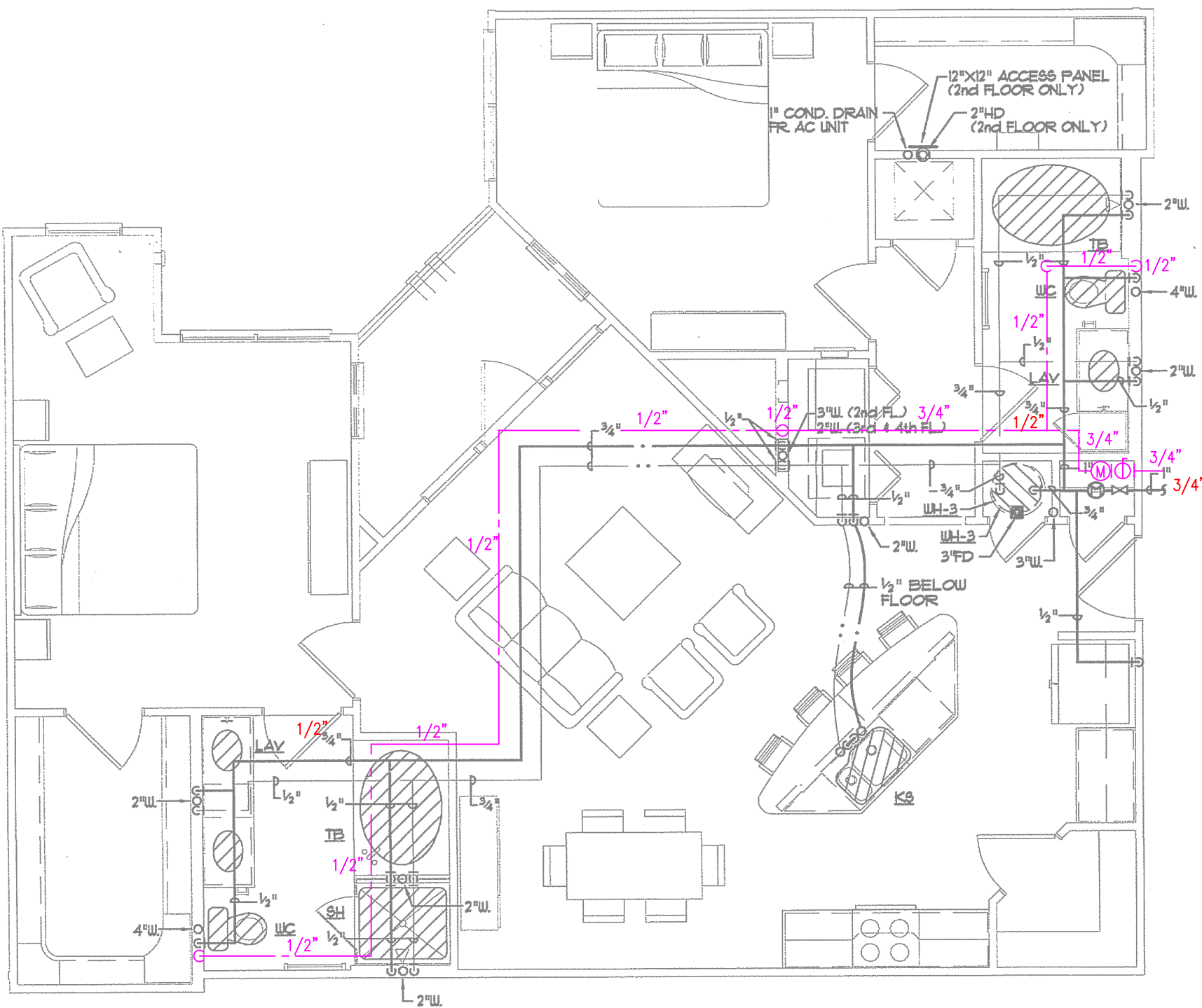
1 UNIT PLAN - B2 - PLUMBING SCALE: 1/4" = 1'-0"
