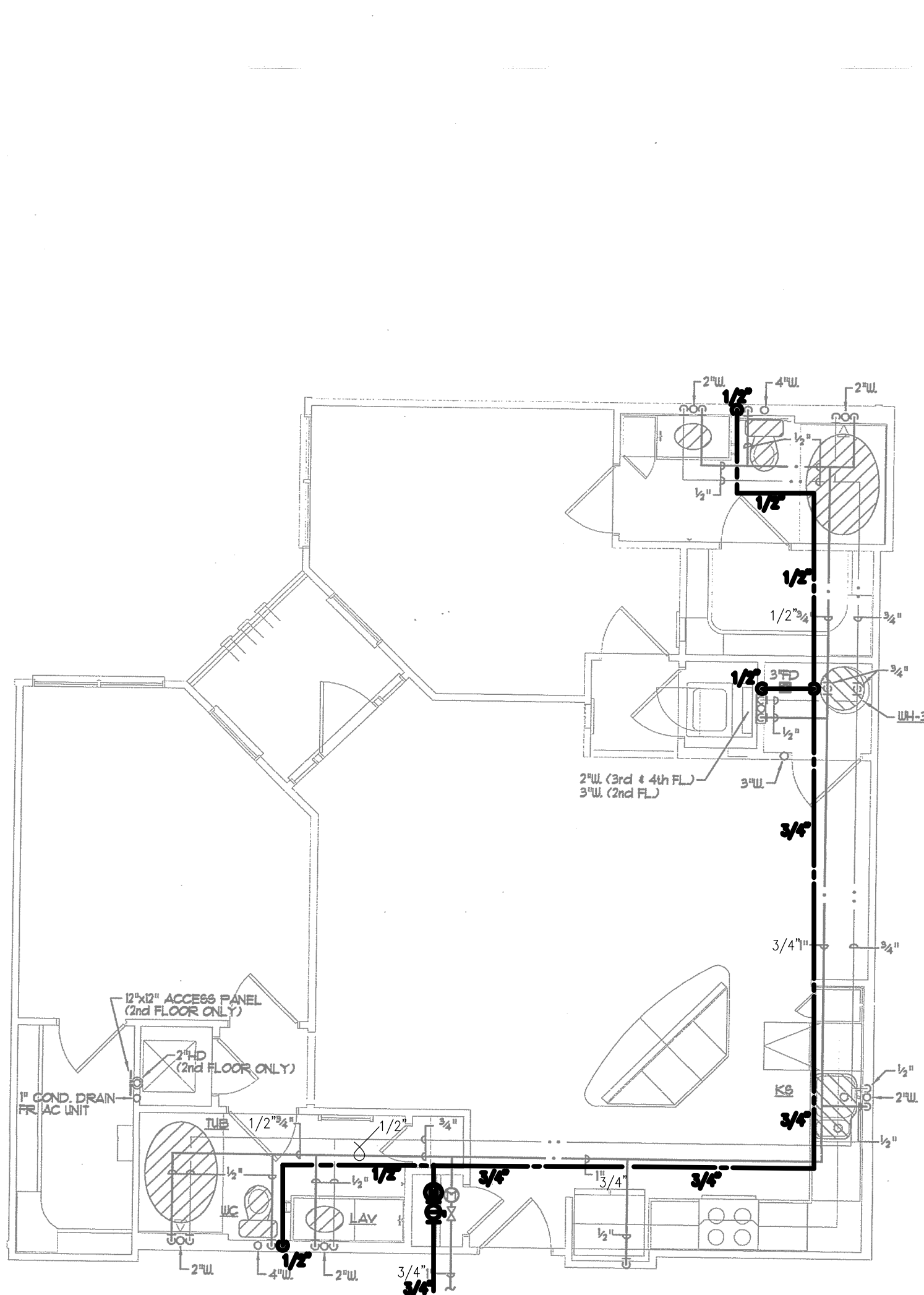
1 UNIT PLAN - B1 - PLUMBING SCALE: 1/4" = 1'-0"
