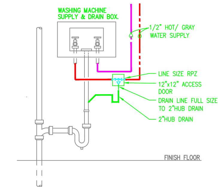
RPZ/HUB DRAIN @ WASHER BOX SCALE: NOT TO SCALE
