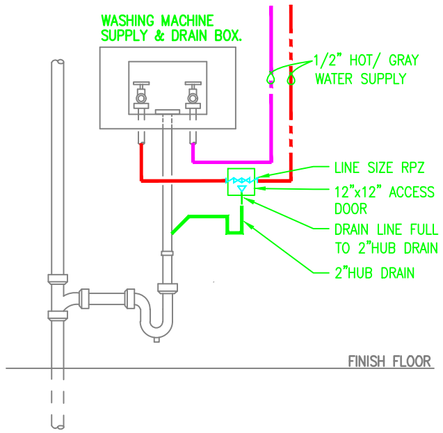
RPZ/HUB DRAIN @ WASHER BOX SCALE: NOT TO SCALE
