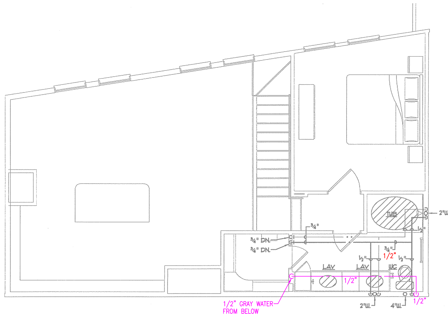
2 UNIT PLAN - A2L- UPPER - PLUMBING SCALE: 1/4" = 1'-0"
