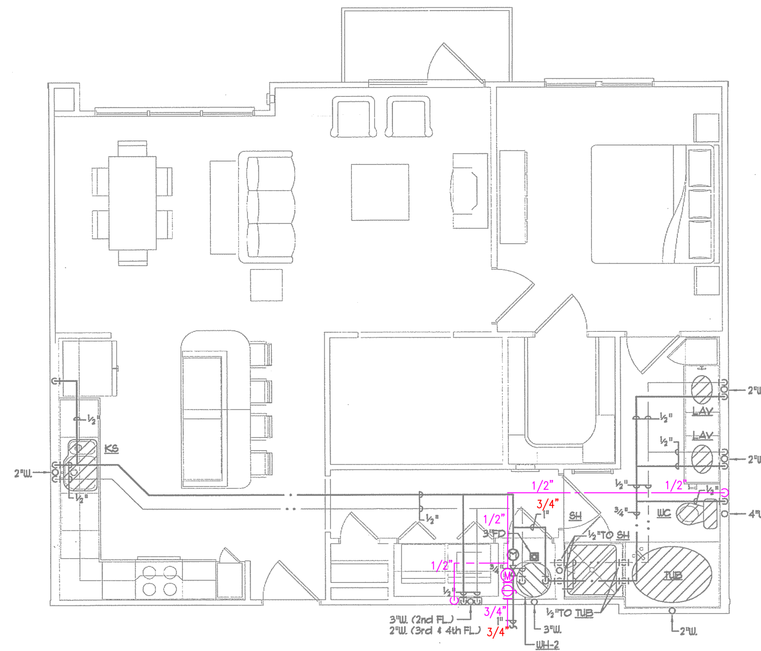
2 UNIT PLAN - A3E - PLUMBING SCALE: 1/4" = 1'-0"
