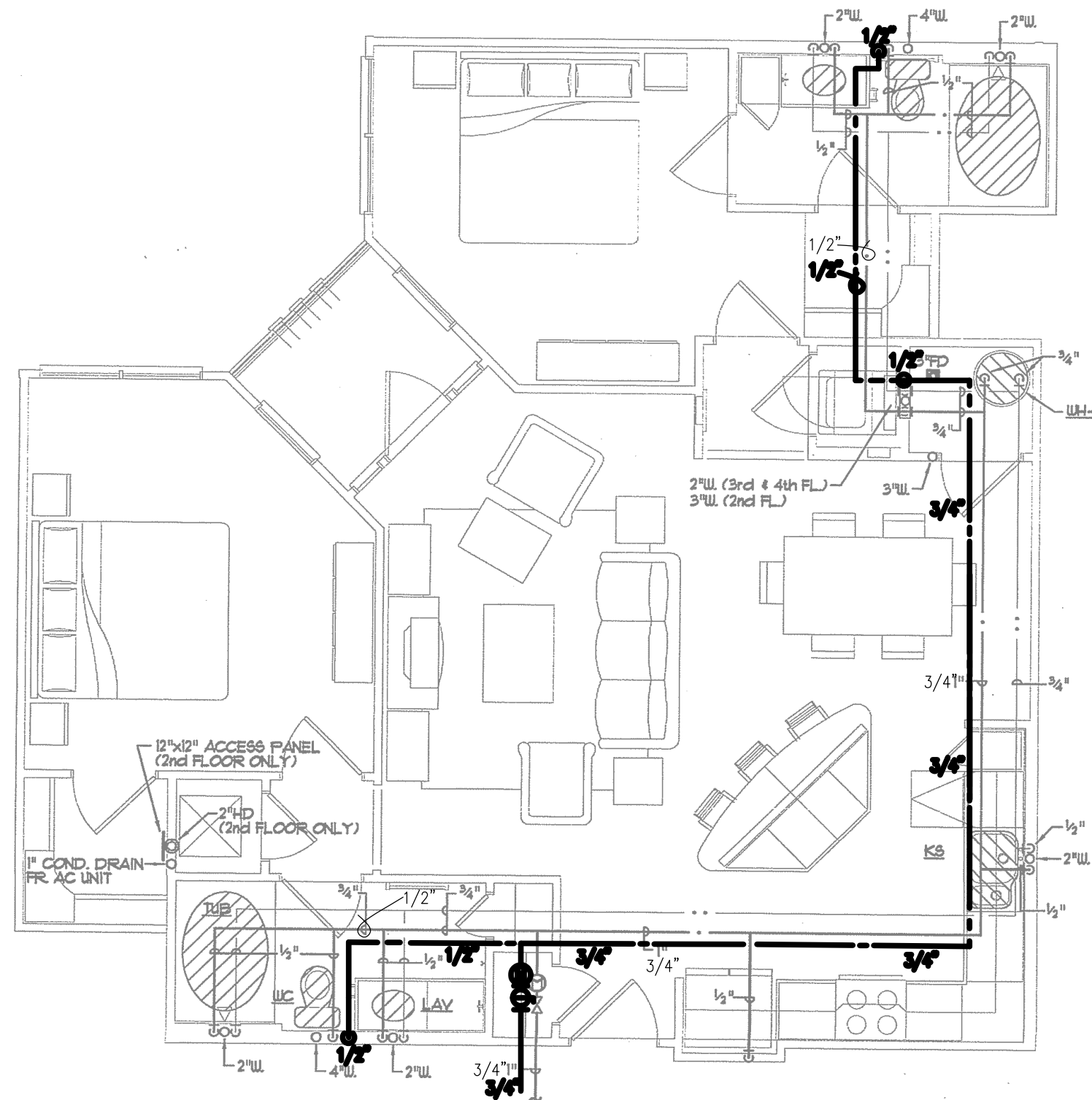
3 UNIT PLAN - B1B - PLUMBING SCALE: 1/4" = 1'-0"
