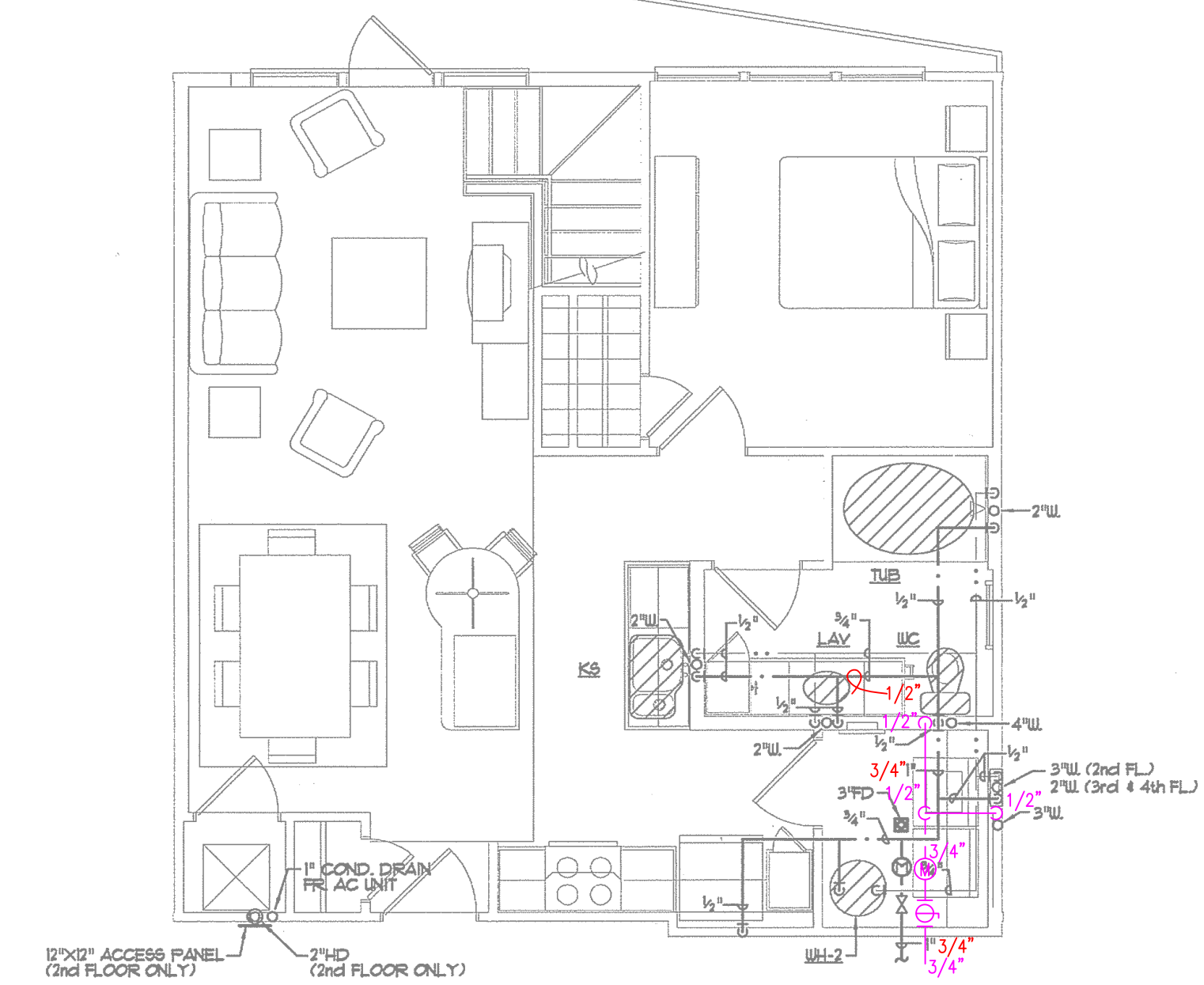
2 UNIT PLAN - A1LA-1 - PLUMBING SCALE: 1/4" = 1'-0"
