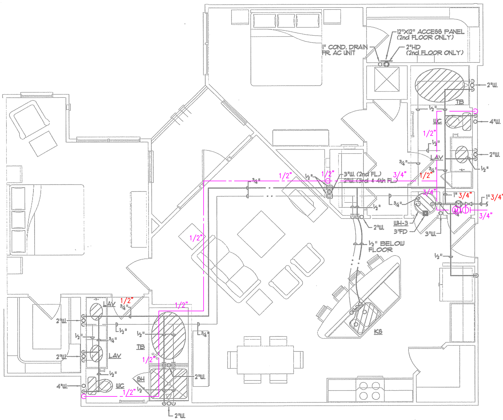
1 UNIT PLAN - B2D - PLUMBING SCALE: 1/4" = 1'-0"
