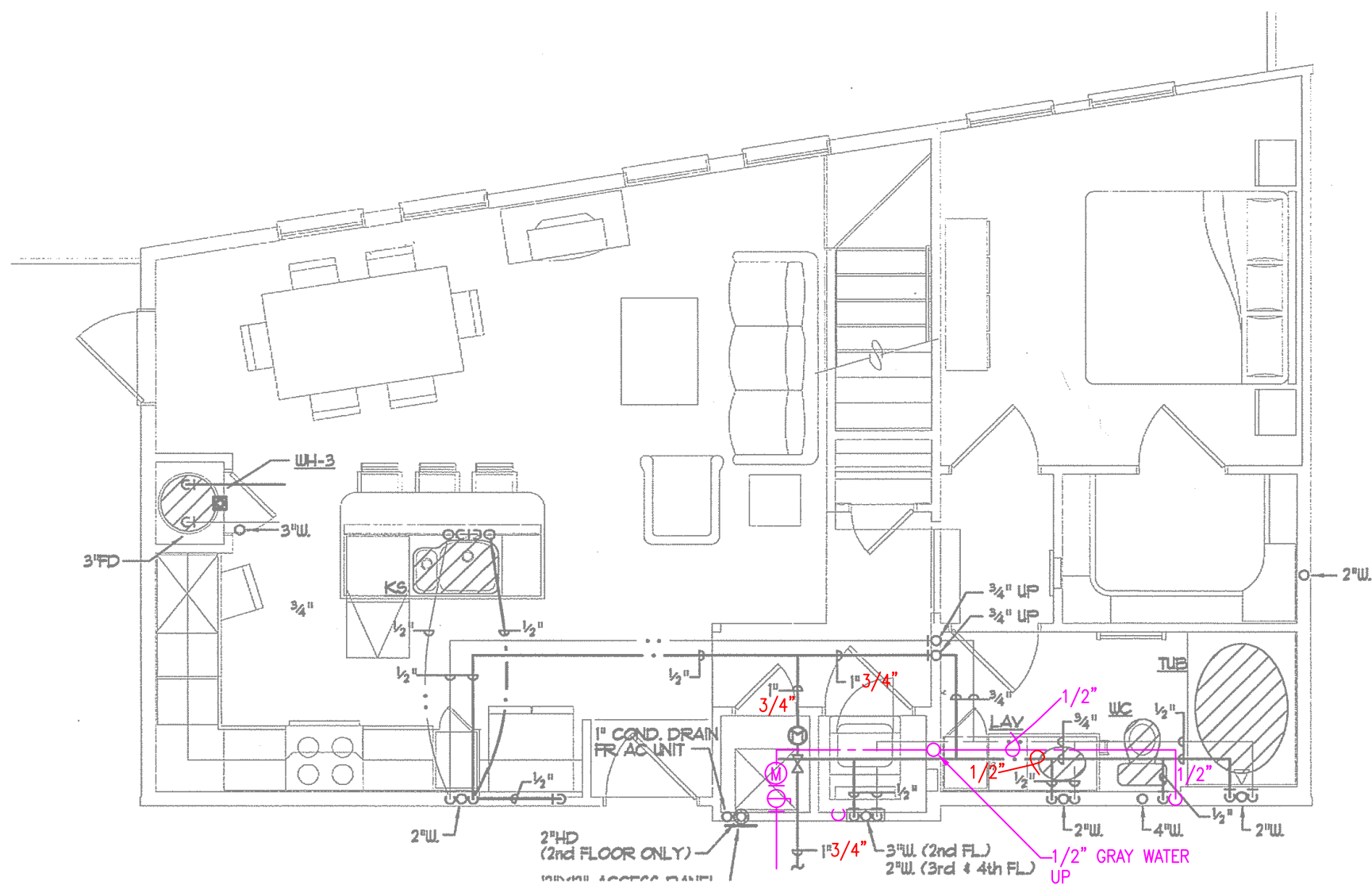
1 UNIT PLAN - A2L - LOWER - PLUMBING SCALE: 1/4" = 1'-0"
