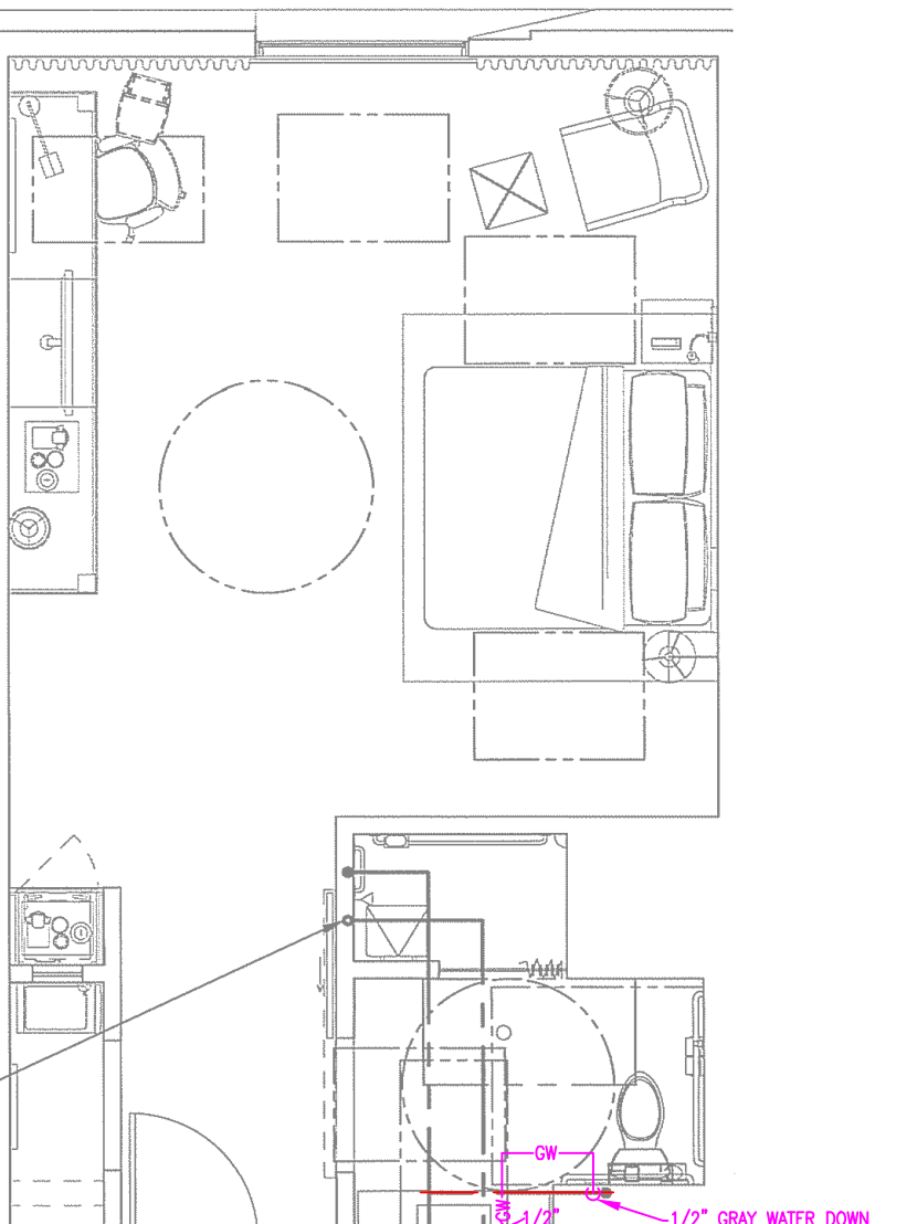
4 KING ACCESSIBLE 1/4" = 1'-0"
