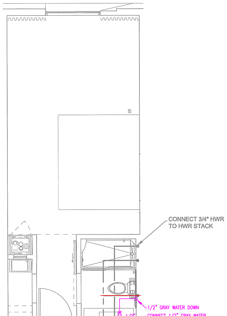
2 KING SUITE 1/4" = 1'-0"
