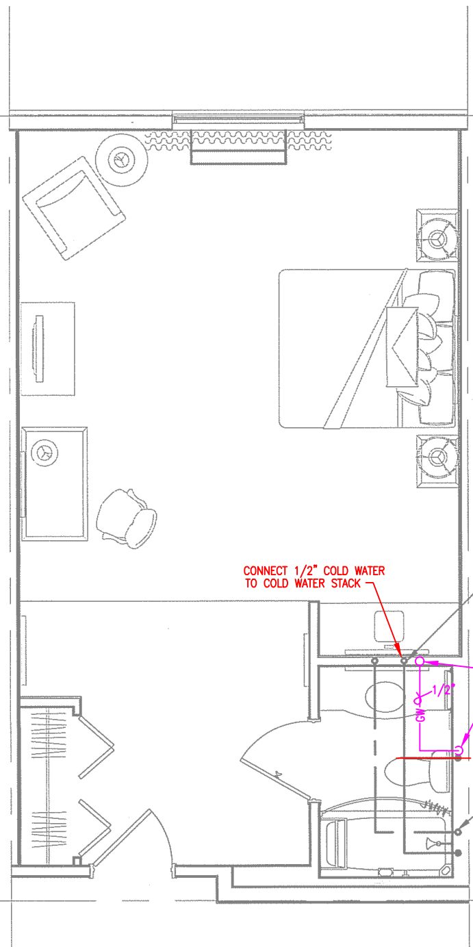
3 KING ENLARGED 1/4" = 1'-0"
