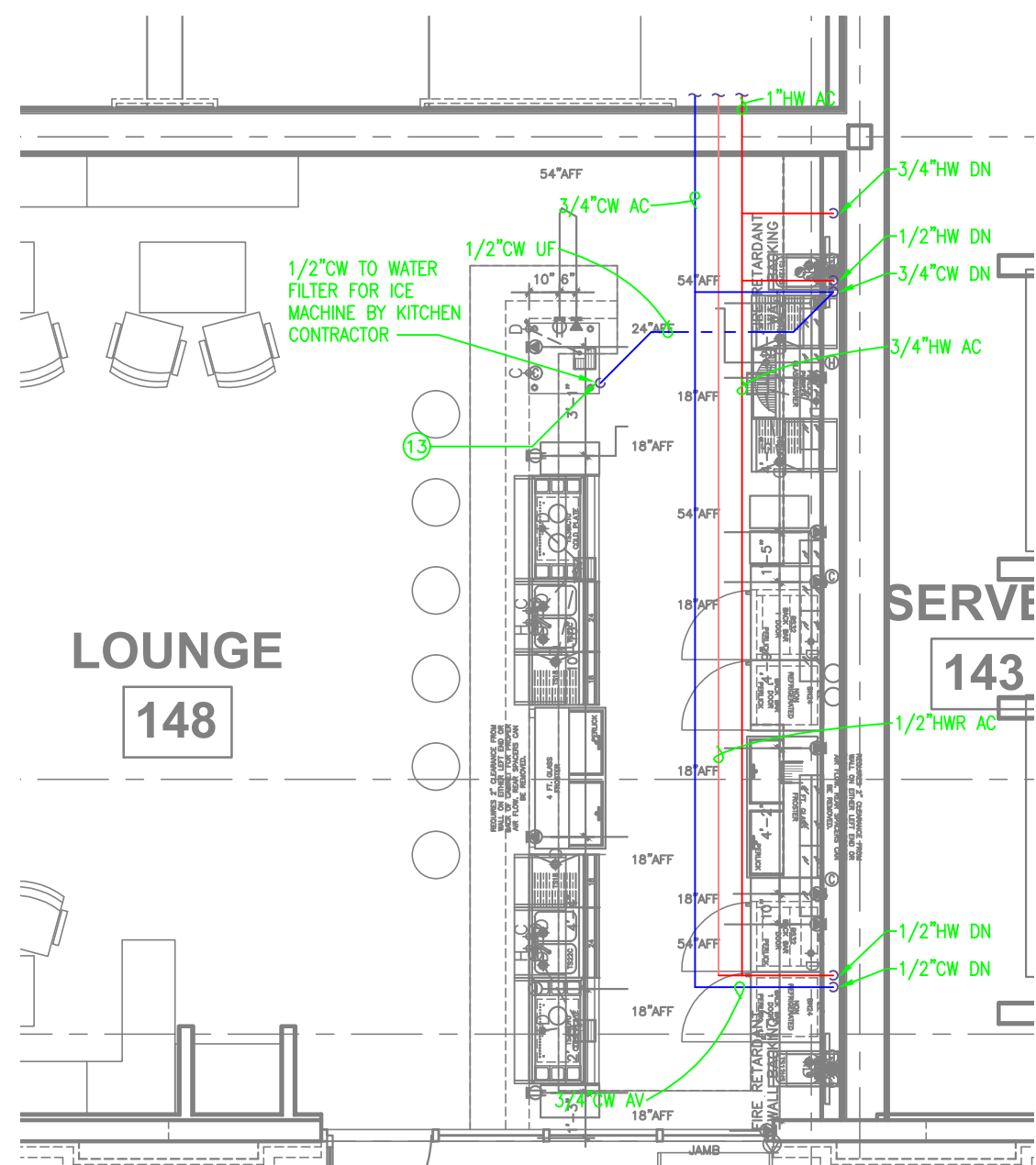
2 PLUMBING ENLARGED SATALLITE BAR PLAN CW, HW, HWR & NAT GAS SCALE: 1/4"=1'-0"
