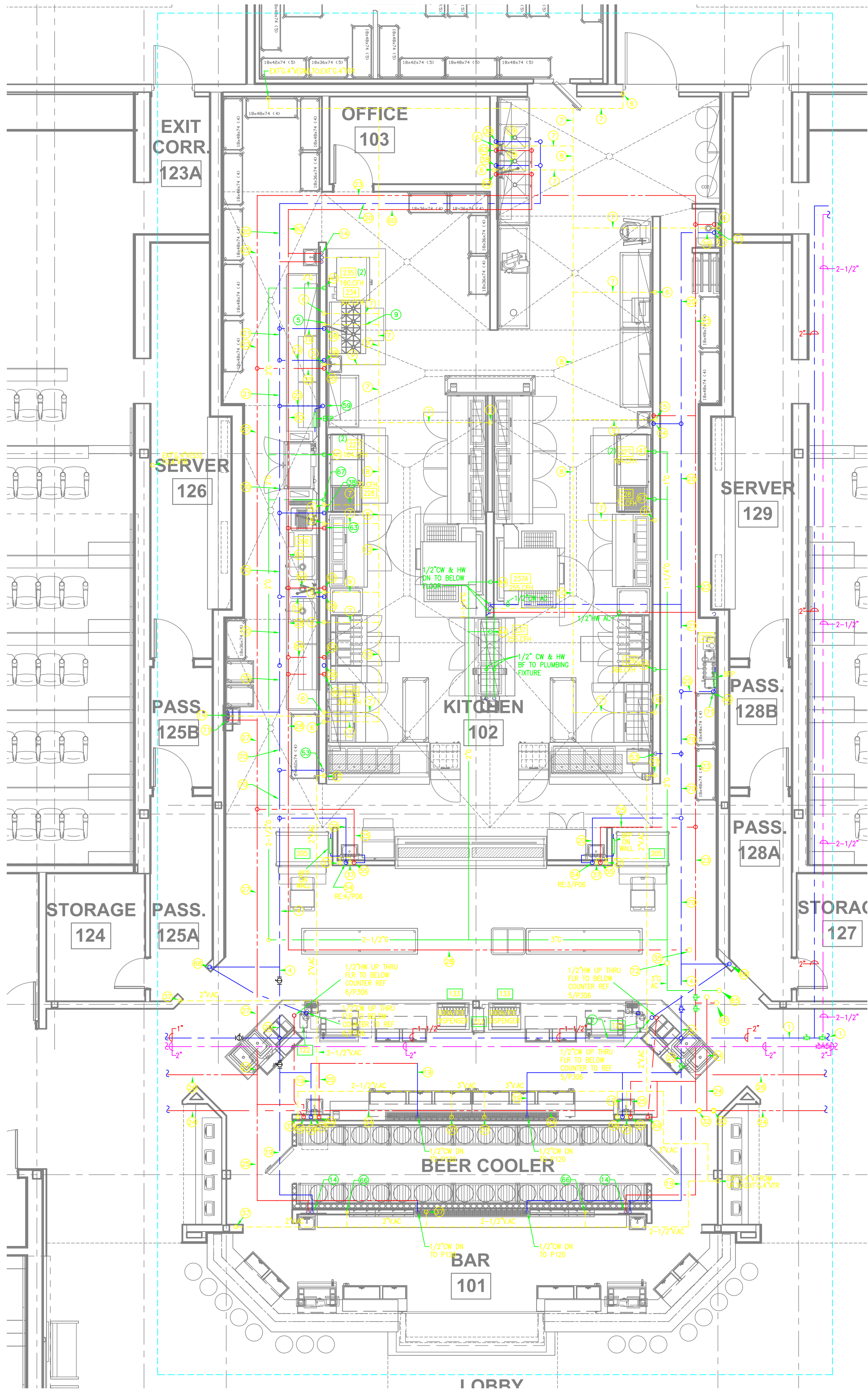
1 PLUMBING ENLARGED KITCHEN PLAN – CW, HW, HWR & NAT GAS SCALE: 1/4"=1'-0"
