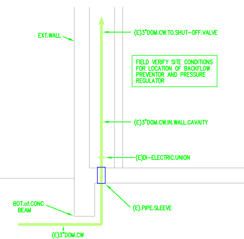
5 EXT'G DOMESTIC CW ENTRY DETAIL NOT TO SCALE
