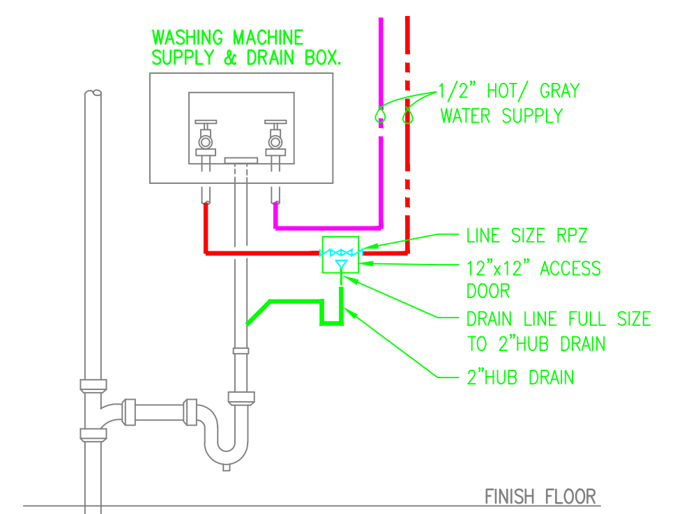
RPZ/HUB DRAIN @ WASHER BOX SCALE: NOT TO SCALE
