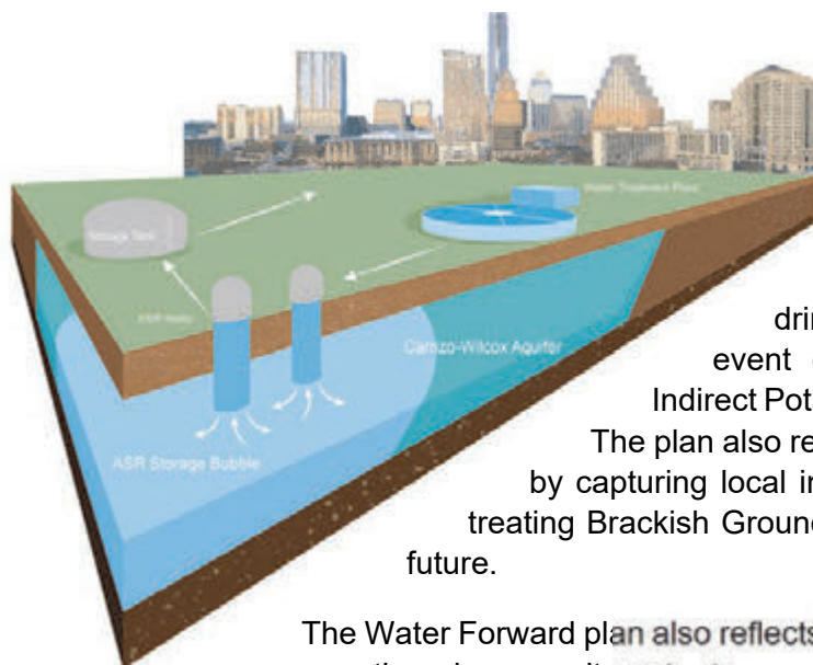
Figure 1-3. Aquifer Storage and Recovery
